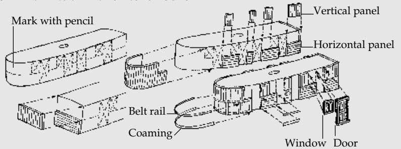
FIG. 10 – Main Cabin Panel Construction
